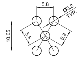
ENLARGED DETAIL AT - A
